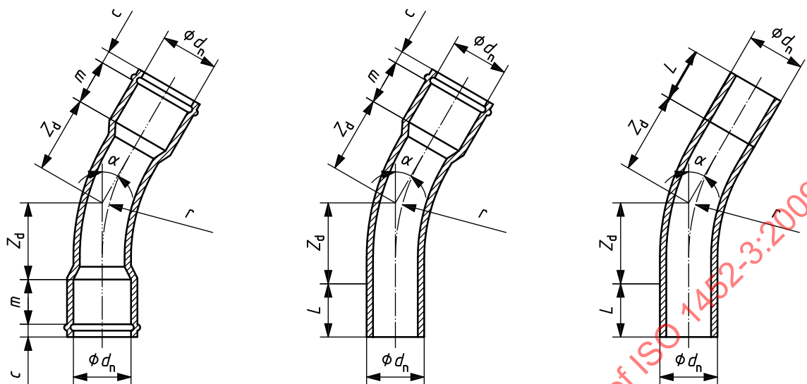
Figure 17 — Typical bends made from pipes
