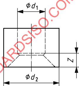
a) Reducing bush, short
