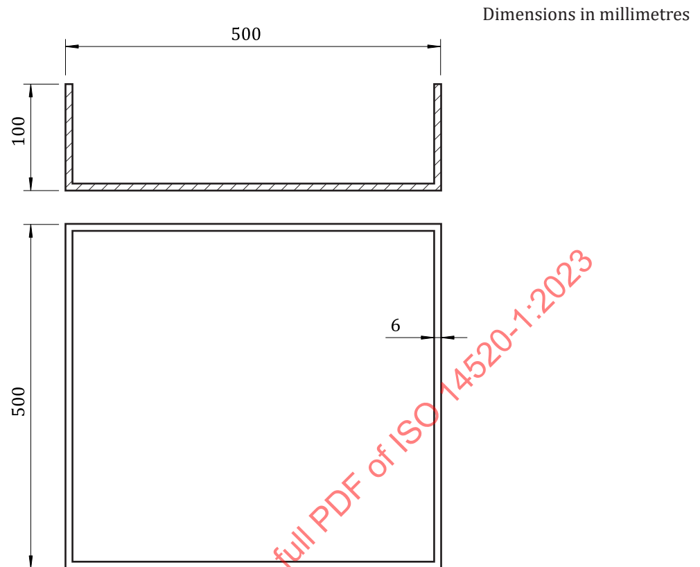
Figure C.7 — Pan geometry for the wood crib and heptane pan fire test
