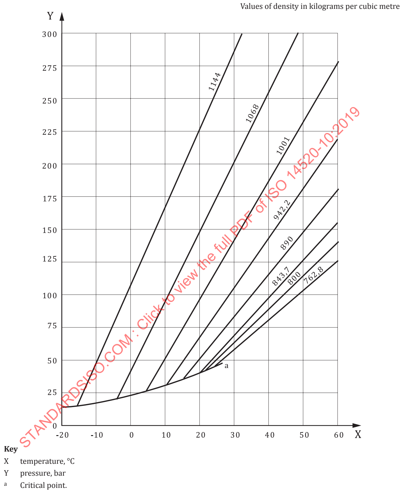
Figure 1 — Temperature/pressure graph for HFC 23
