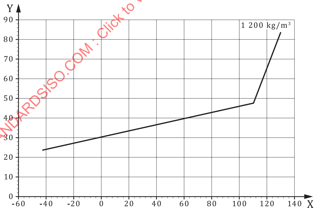
Figure 1 — Temperature/pressure graph for FK-5-1-12 superpressurized with nitrogen 25 bar at 20 °C
