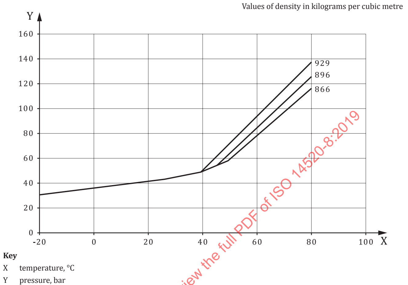
Figure 2 — Temperature/pressure graph for HFC 125 pressurized with nitrogen at 42 bar and 22 °C
