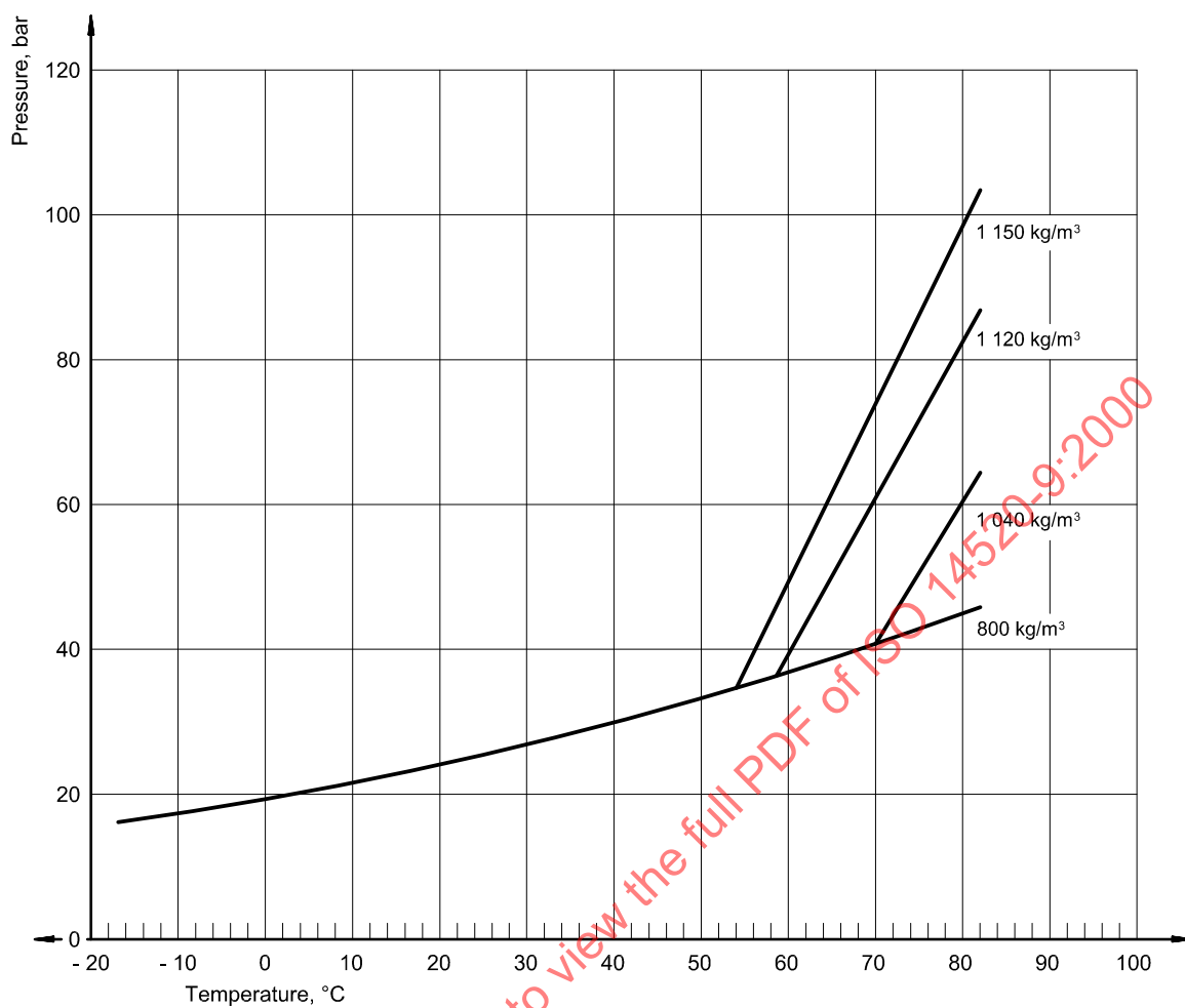
Figure 1 — Temperature/pressure graph for HFC 227ea superpressurized with nitrogen to 25 bar at 21 °C
