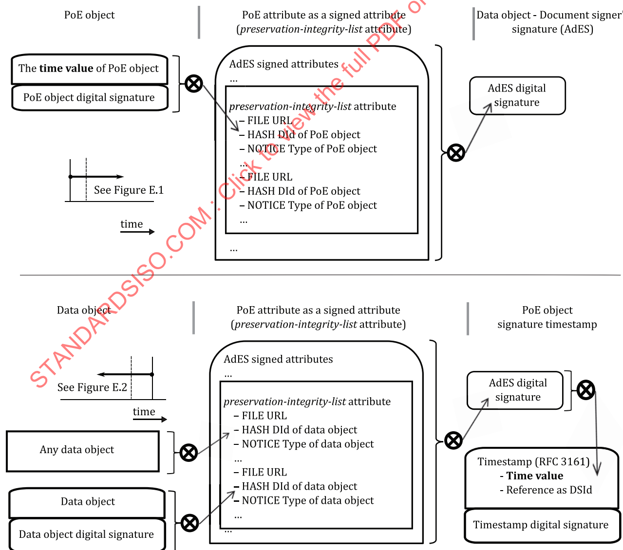
Figure 6 — Example of the preservation-integrity-list attribute as a signed attribute
