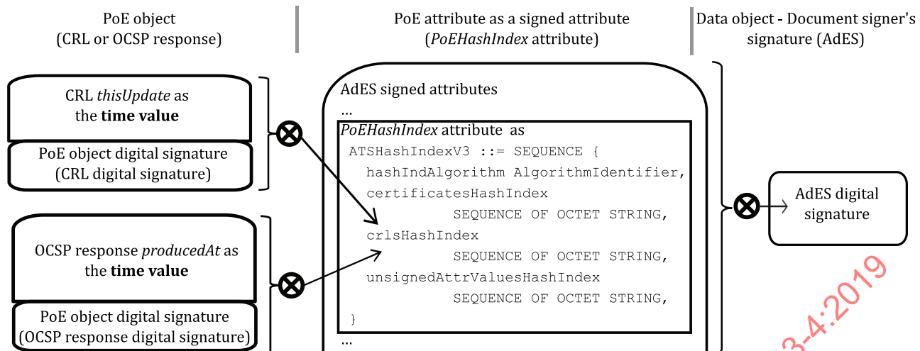
Figure 5 — Signature created after the thisUpdate time of CRL or producedAt of OCSF response
