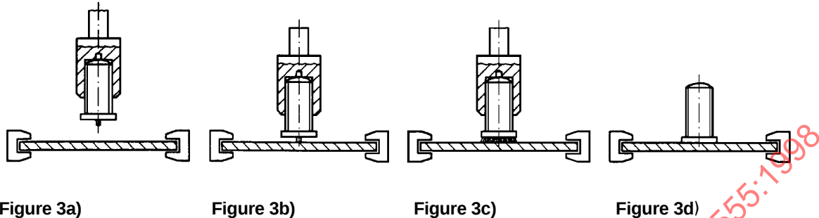
Figure 3: Capacitor discharge stud welding with tip ignition - Main phases of the welding process
