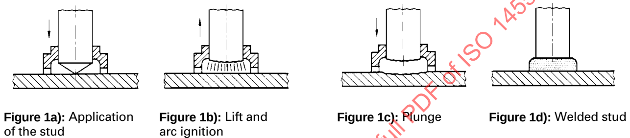
Figure 1: Drawn arc stud welding, sequence of operations
