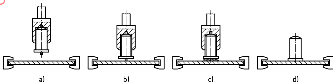
Figure A.2 — Capacitor discharge stud welding with tip ignition — Main phases of the welding process
