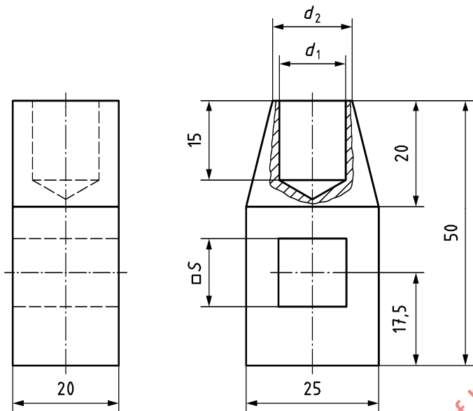
b) Test tool for bend testing
