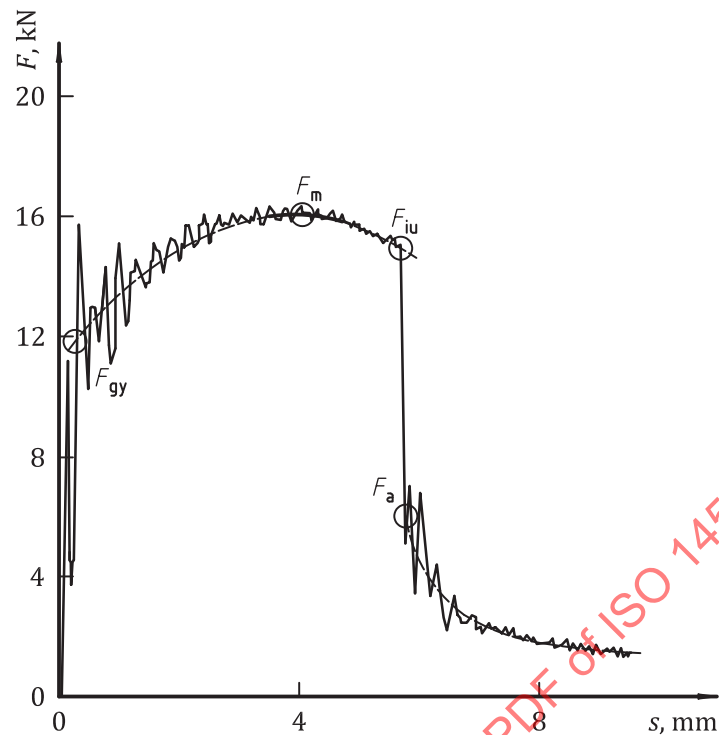
Figure 3 — Determination of the characteristic values of force
