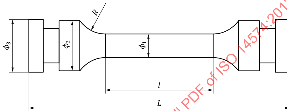
Figure 2 — Type 2 test specimen
