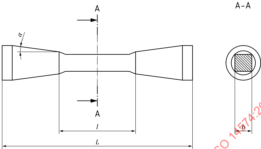
Figure 3 — Type 3 test specimen
