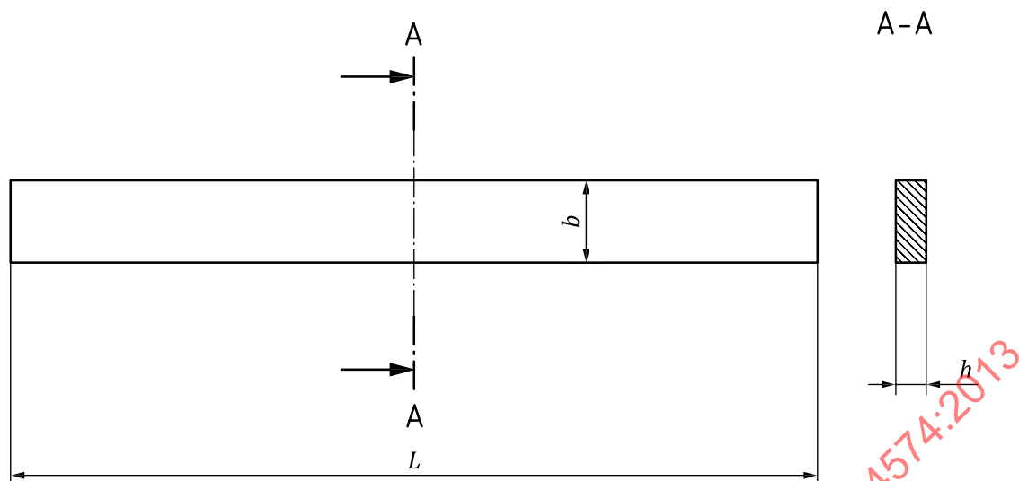
Figure 6 — Type 6 test specimen
