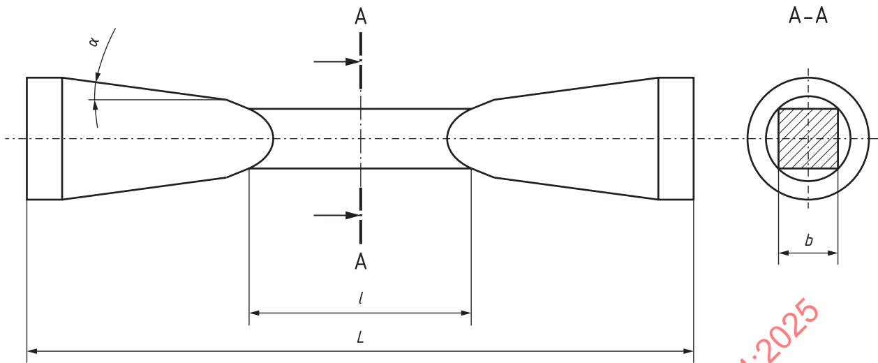
Figure 3 — Type 3 test specimen
