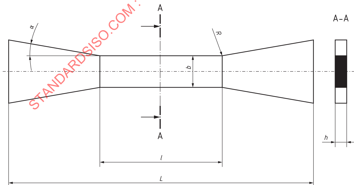
Figure 1 — Type 1 test specimen
