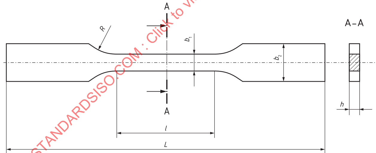
Figure 4 — Type 4 test specimen
