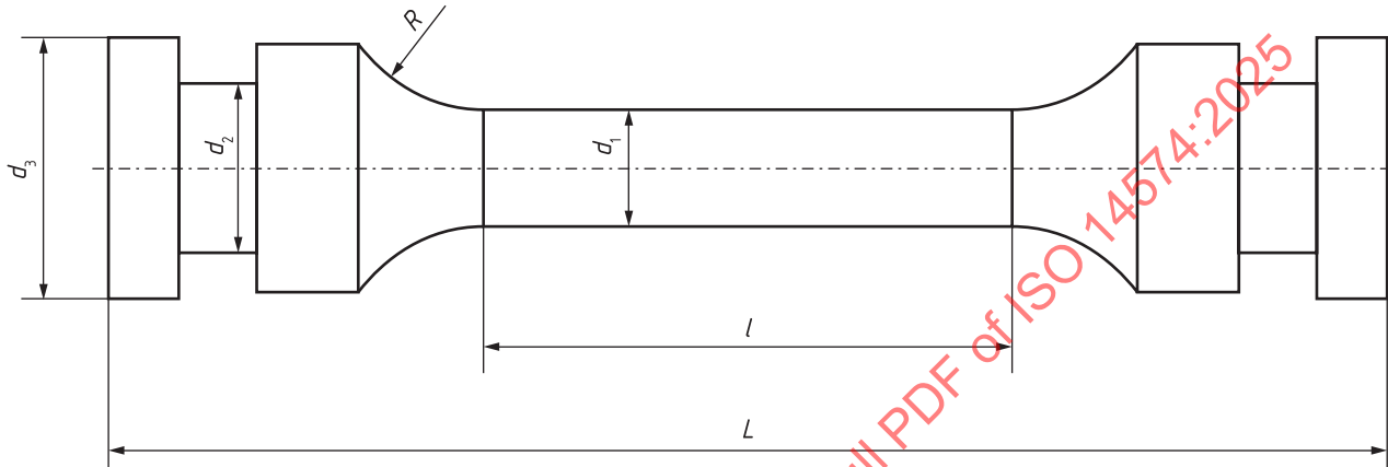
Figure 2 — Type 2 test specimen
