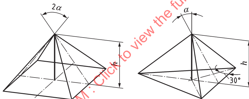
Figure A.1 — Shape of indenters for determination of HM
