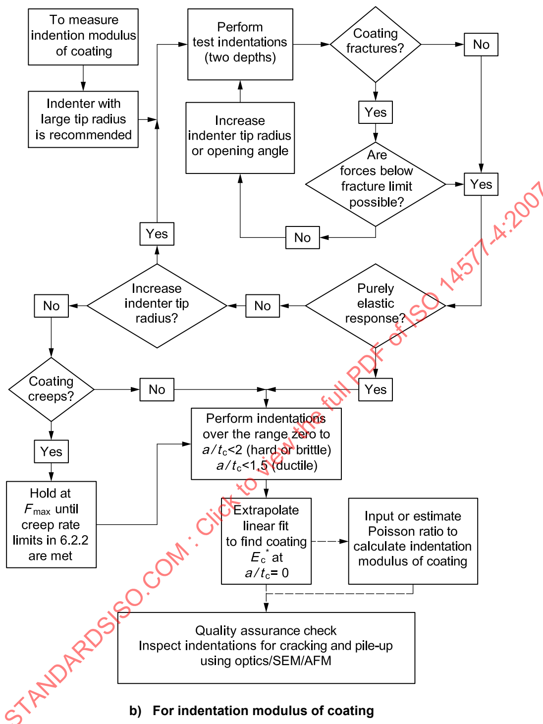
Figure 2 — Flow chart for selection of indenter geometry and indentation parameters to measure coating properties
