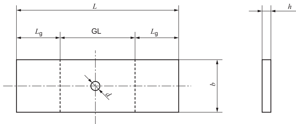
Figure 2 — Open-hole tension test specimen
