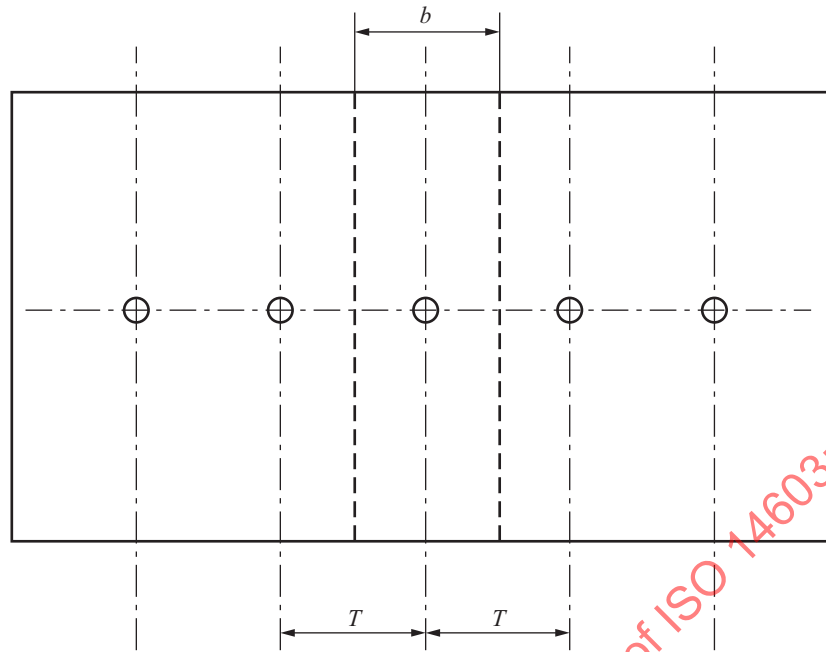
Figure 3 — Schematic drawing illustrating the definition of the minimum distance between holes in a structural component with aligned holes
