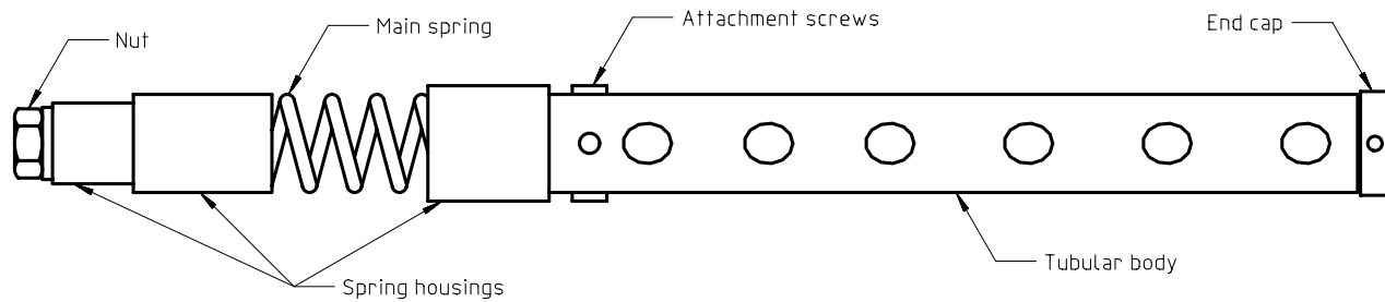
Figure 3 — Specimen-loading tube
