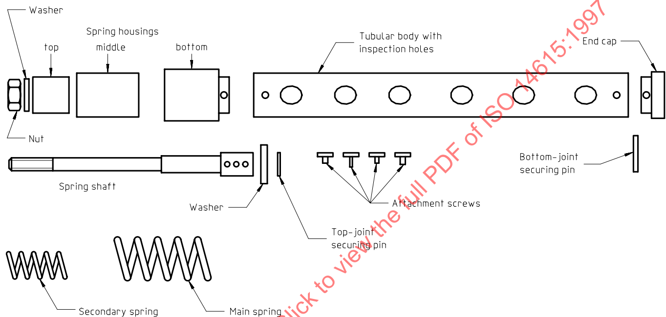
Figure 4 — Components of specimen-loading tube
