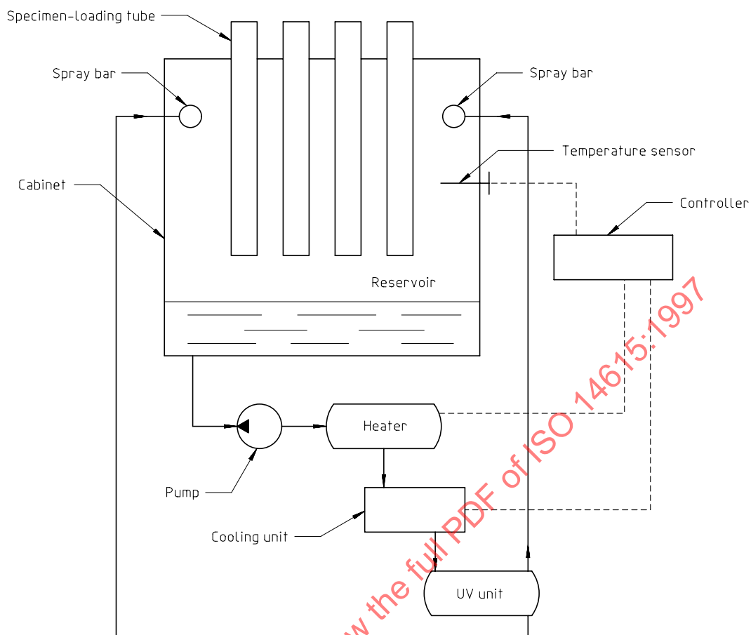
Figure 1 — Schematic diagram of apparatus
