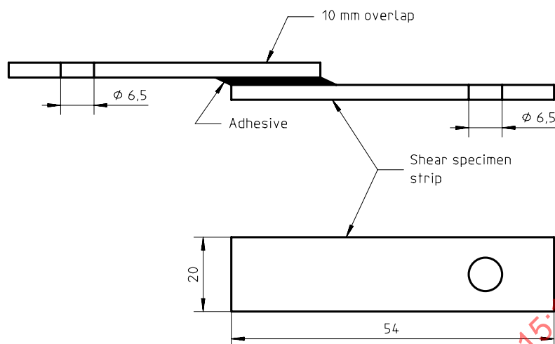
Figure 5 — Typical lap-shear joint
