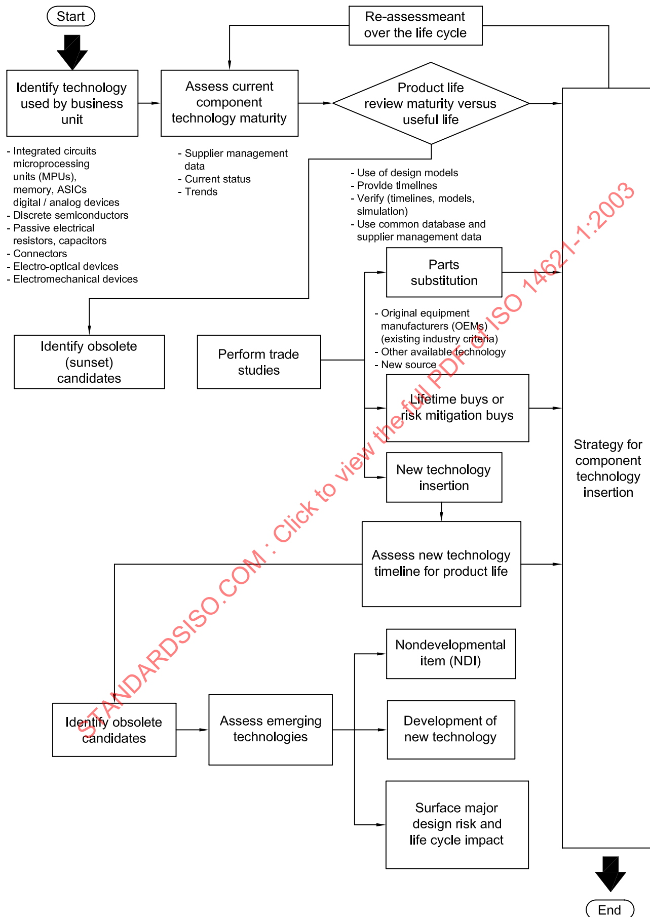
Figure 5 — Technology insertion strategy (road map)
