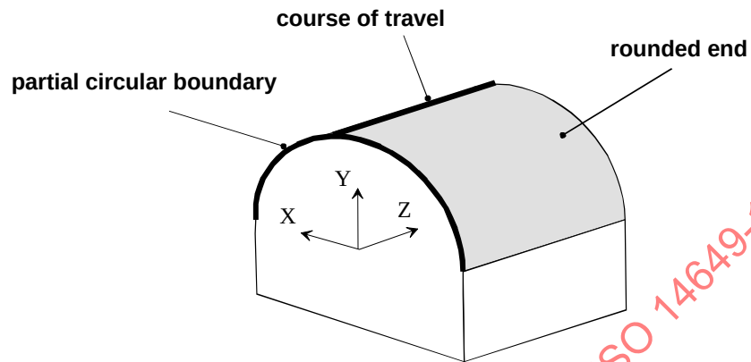
Figure 22 — Rounded end
