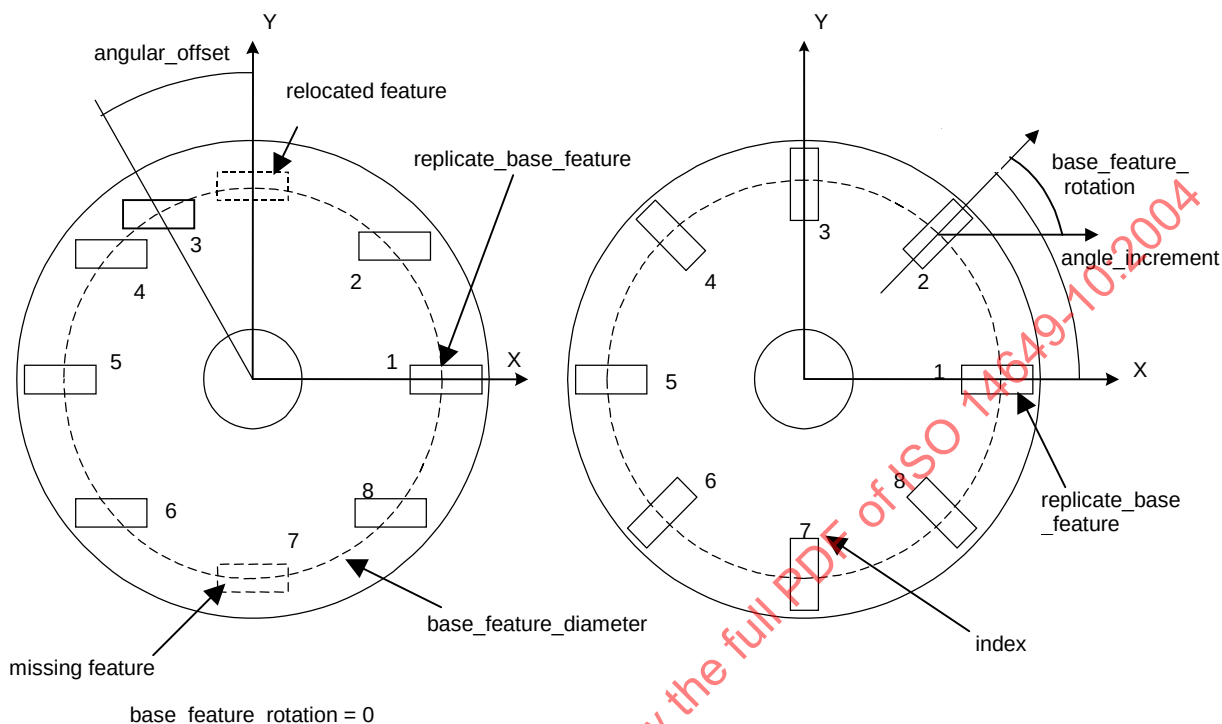
Figure 25 — Circular Pattern
