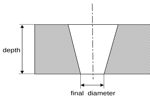
Figure 16 — Diameter taper
