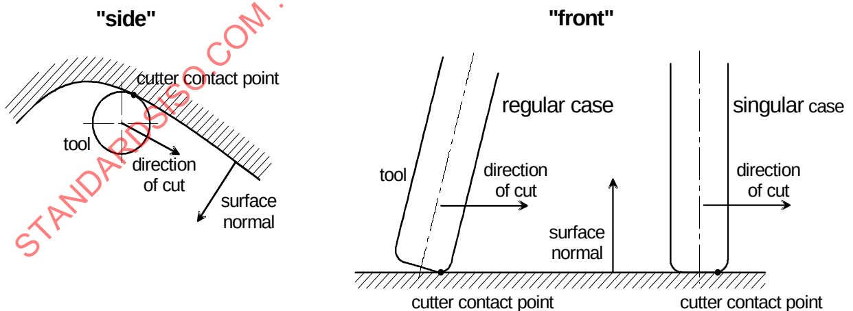
Figure 40 — Contact type
