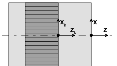
Figure 9: Straight knurl
