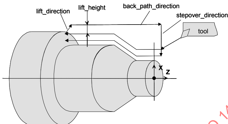
Figure 15: Contour turning
