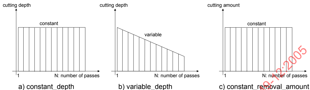
Figure 17: Thread cut depth type for threading
