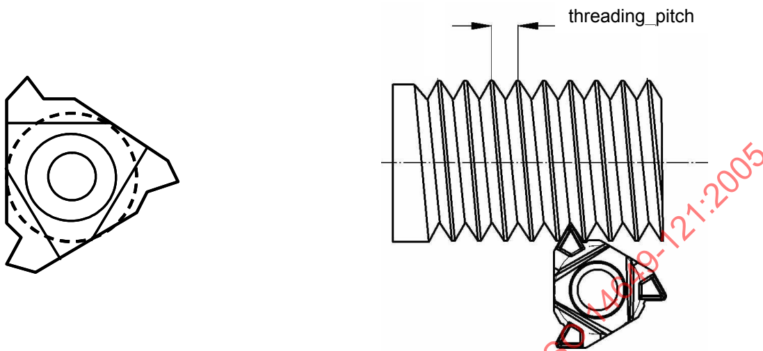
Figure 7: Threading insert.
