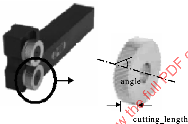
Figure 9: Knurling tool.
