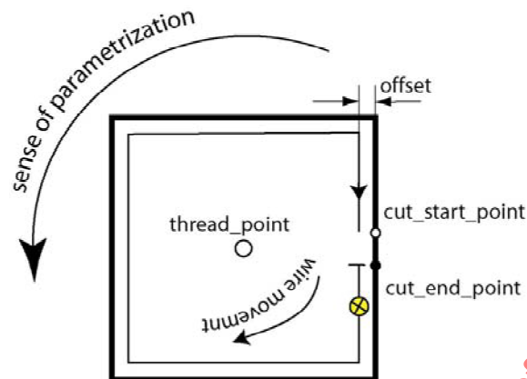
Figure 8 — Backmotion strategy
