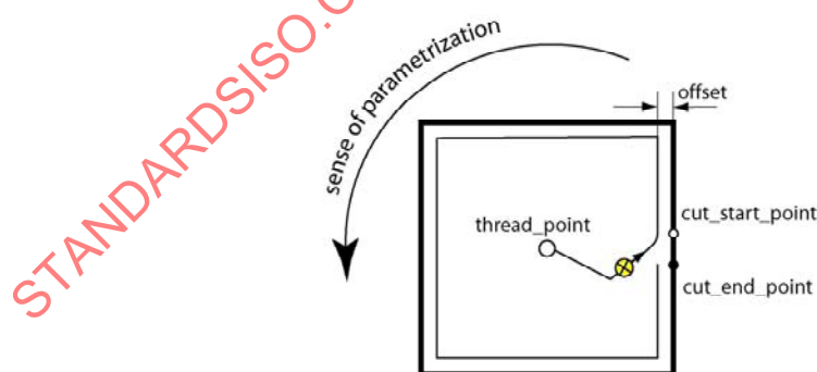
Figure 10 — Along_path_strategy
