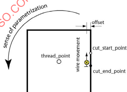
Figure 9 — Cut_through strategy
