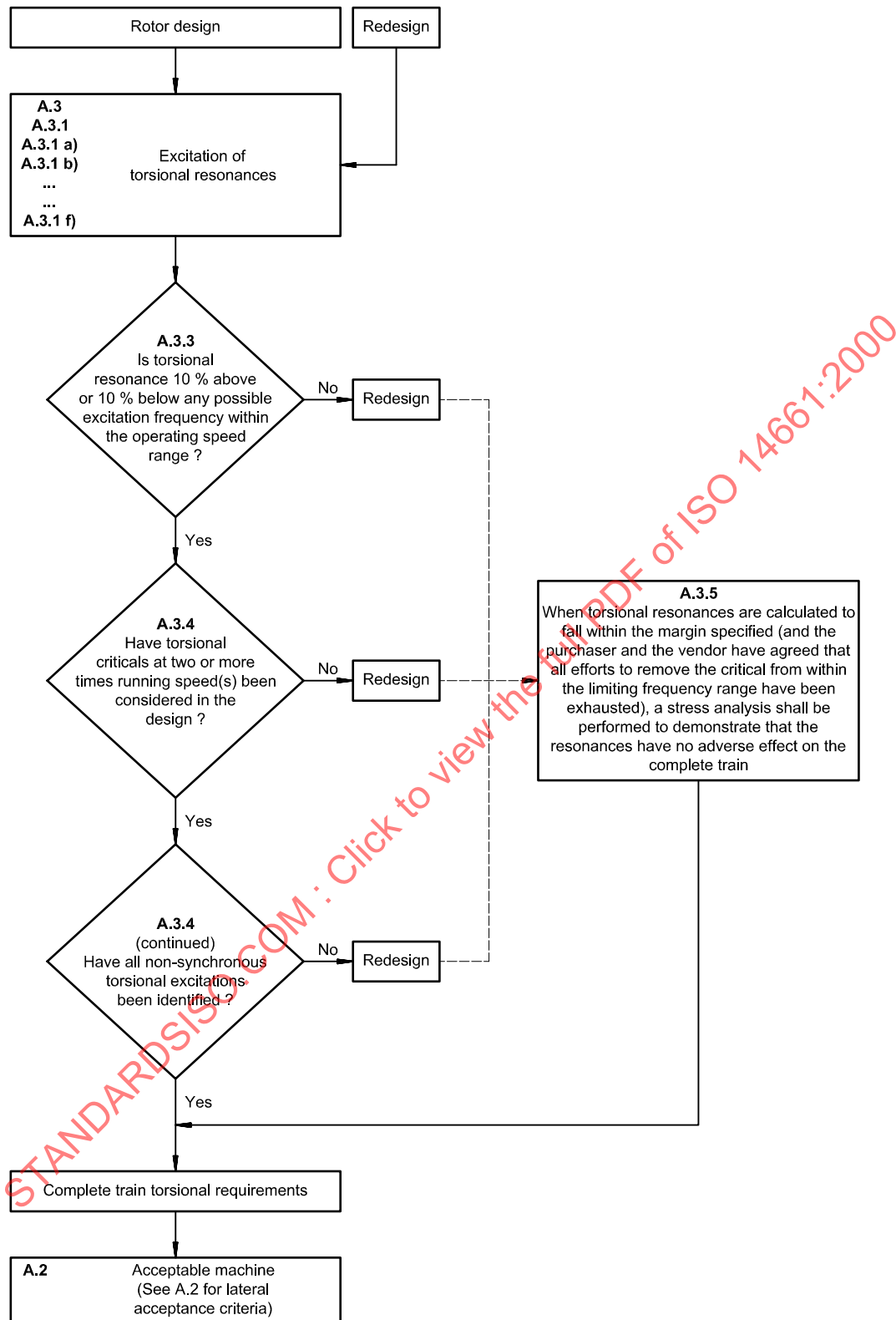
Figure A.4 — Rotor dynamics logic diagram (torsional analysis)
