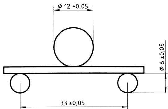
Figure 7 — Test rack
