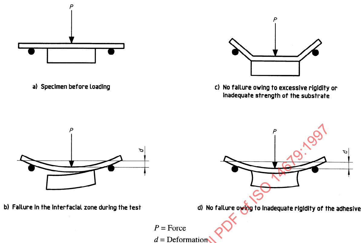
Figure 2 — Principle of the test
