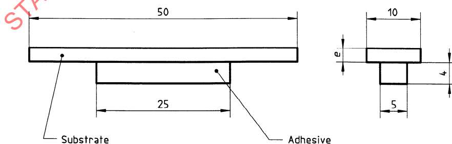
Figure 8 — Specimen
