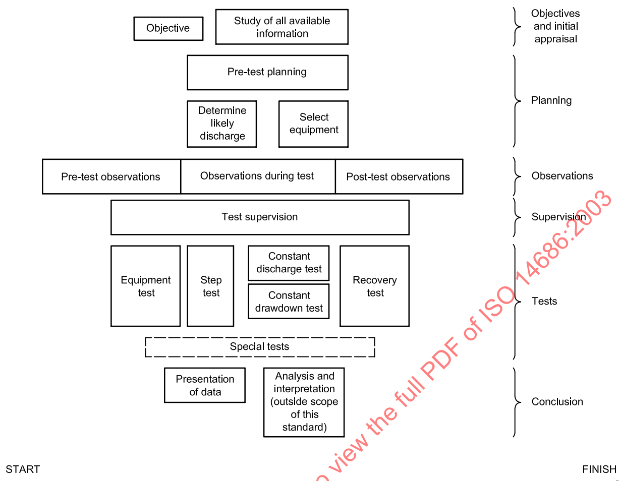
Figure 1 — Typical pumping-test procedure
