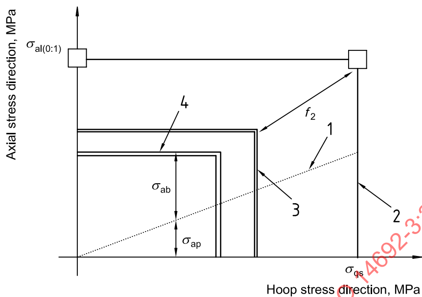
a) Quasi-isotropic GRP joints
