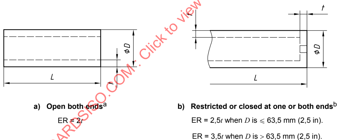
Figure 1 — Equivalent round models — Solids of length L
