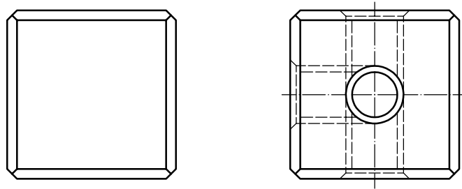
a) Base for thin adhesive
