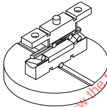
b) Schematic of a fixture with special cradles to hold the bearing rollers
