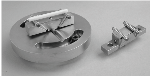
a) Inner pair of bearing rollers (on the right) are parallel and articulate together as a pair in a cradle assembly
