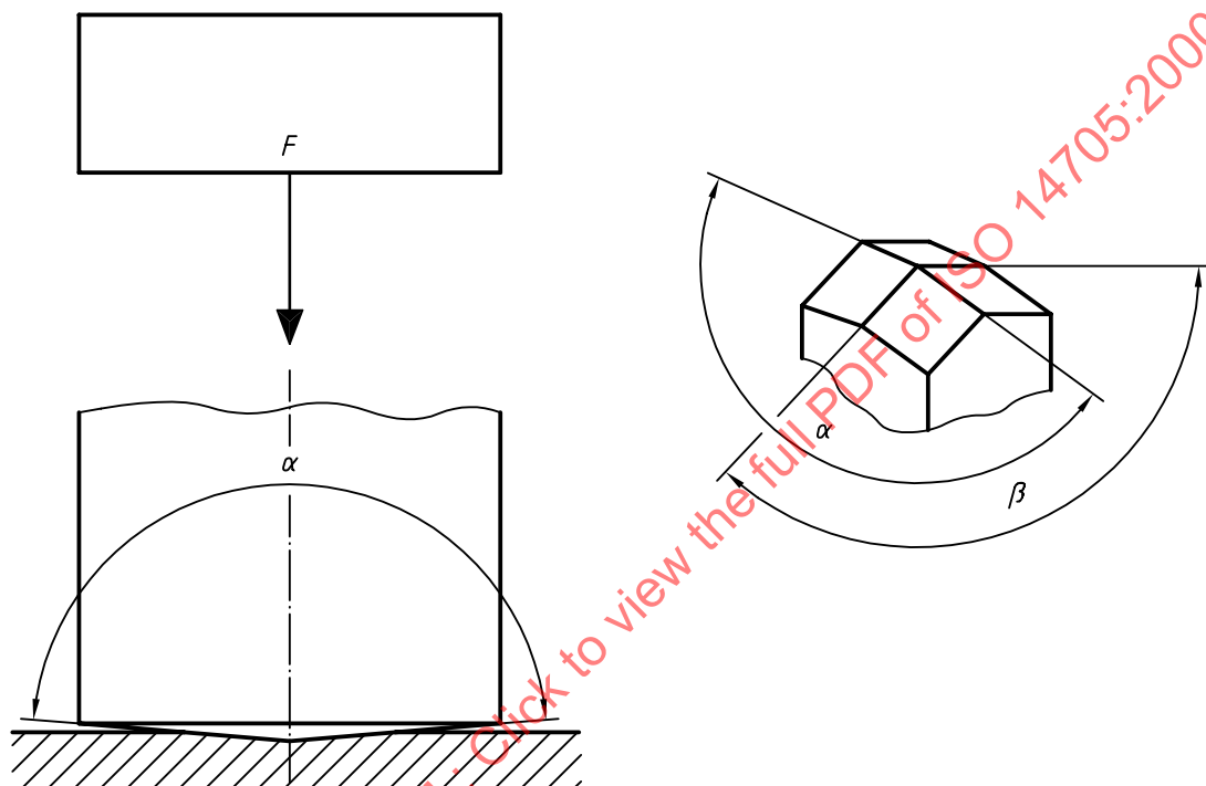
Figure 6 — Knoop indenter
