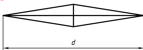
Figure 7 — Knoop indentation
