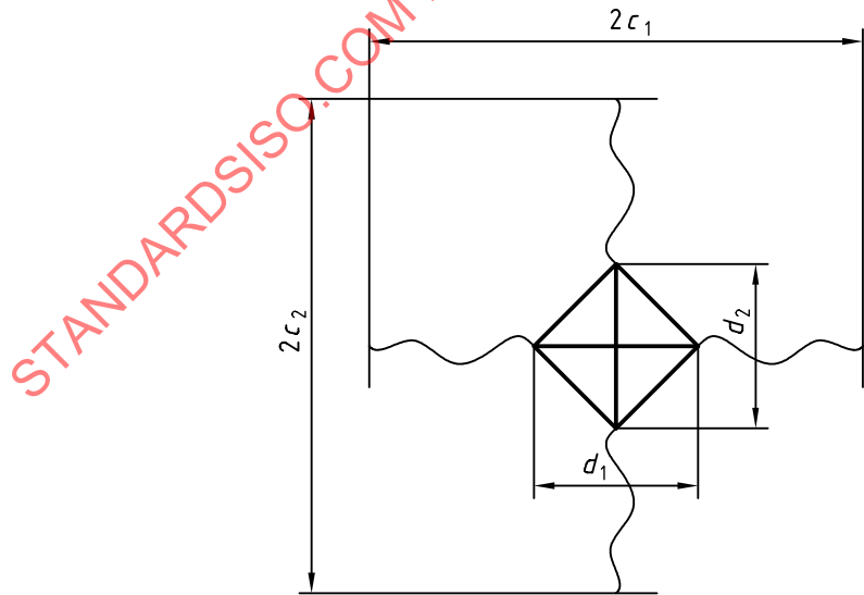
Figure 2 — Vickers indentation
