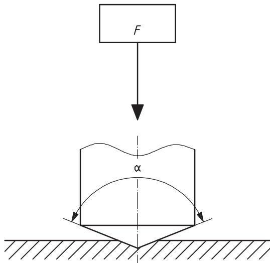
Figure 1 — Vickers indenter (diamond pyramid)
