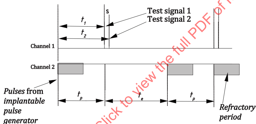
Figure 11 — Measurement of sensing refractory period in triggered (synchronous) mode - A
