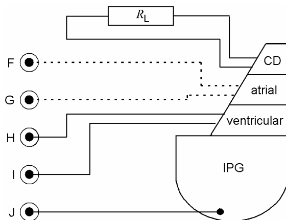
Figure 124 – Common mode connection to multichannel bipolar PULSE generators
