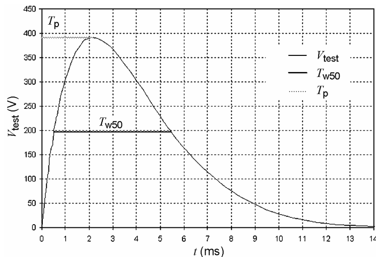
Figure 107 — Damped sinus DEFIBRILLATION waveform
