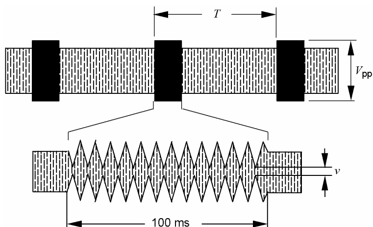
Figure 129 — Test signal for frequencies between 10 MHz and 450 MHz
