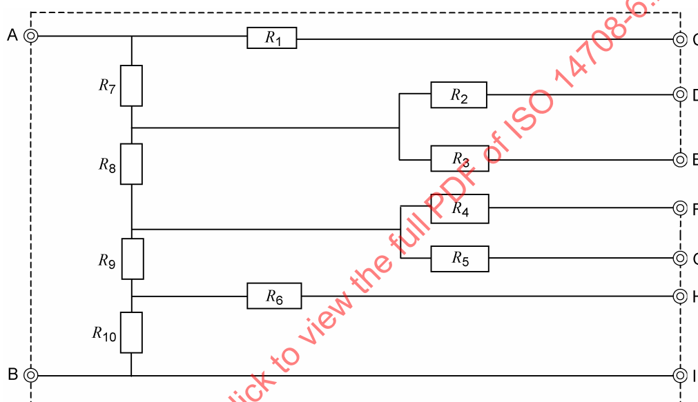
Figure 110 — Resistor network for Test 1 and Test 2
