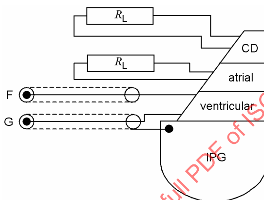
Figure 137 — Connection of the PULSE generator
