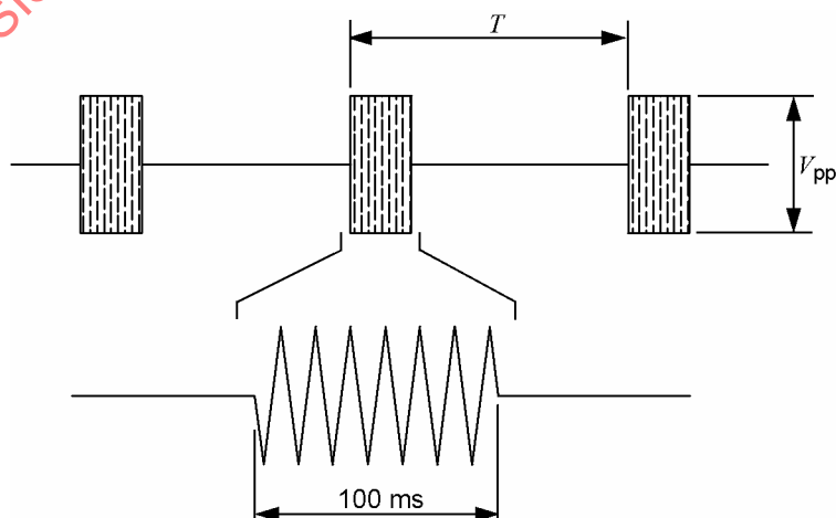
Figure 133 — Modulation 1
