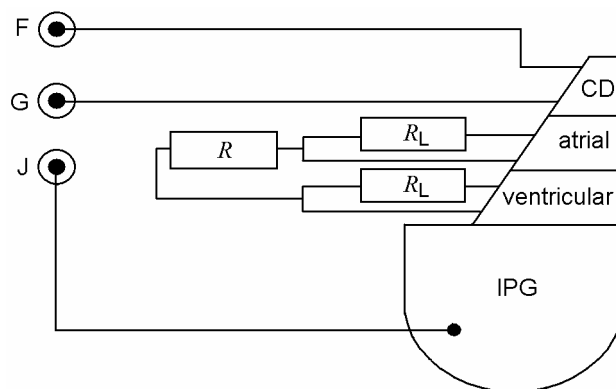
Figure 121 — Common mode connection for CARDIOVERSION/DEFIBRILLATION TERMINALS
