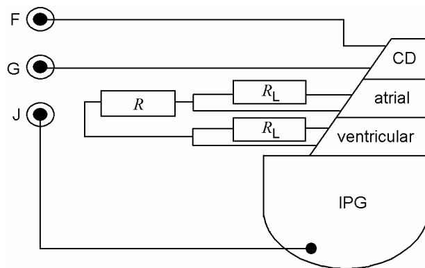
Figure 127 — Common mode connection for CARDIOVERSION/DEFIBRILLATION TERMINALS
