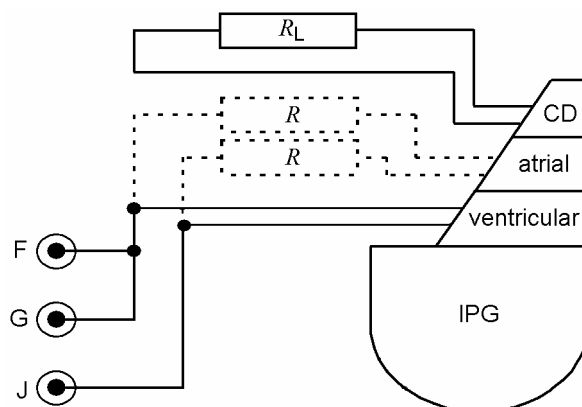
Figure 120 — Differential mode connection to multichannel bipolar PULSE generators
