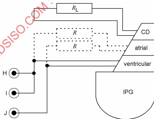
Figure 125 — Differential mode connection to multichannel bipolar PULSE generators
