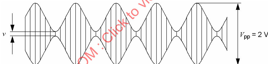
Figure 117 — Test signal 2
