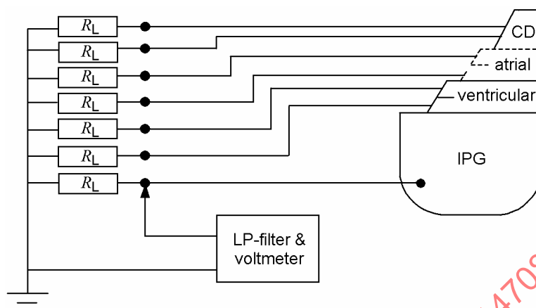
Figure 103 — Test set-up for measurement of electrical neutrality
