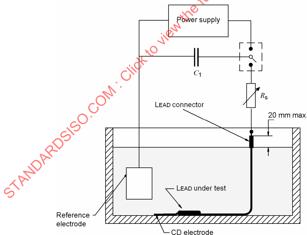
Figure 114 — Conductor current integrity test fixture
