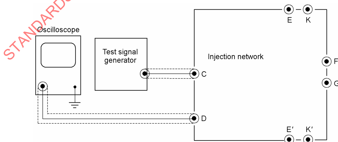
Figure 130 — Test set-up to check for induced malfunction at high frequency
