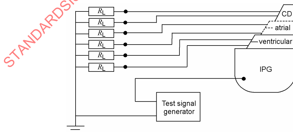
Figure 113 — Test set-up for proof of protection from high-frequency currents caused by surgical equipment
