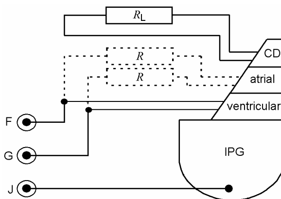
Figure 119 — Common mode connection to multichannel bipolar PULSE generators
