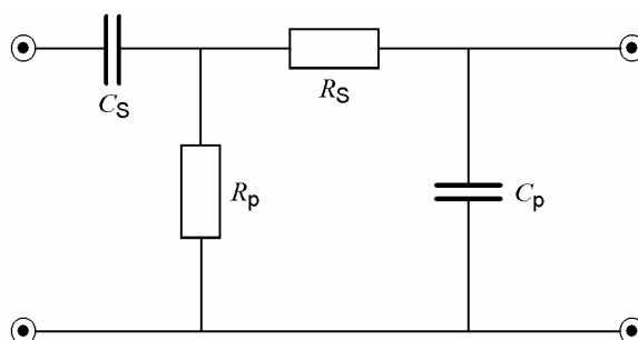
Figure 104 — Band pass filter for a.c. leakage current measurement
