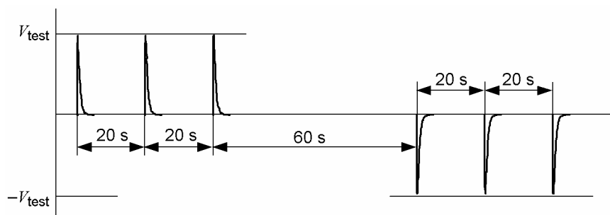
Figure 109 — Timing sequence used for DEFIBRILLATION test
