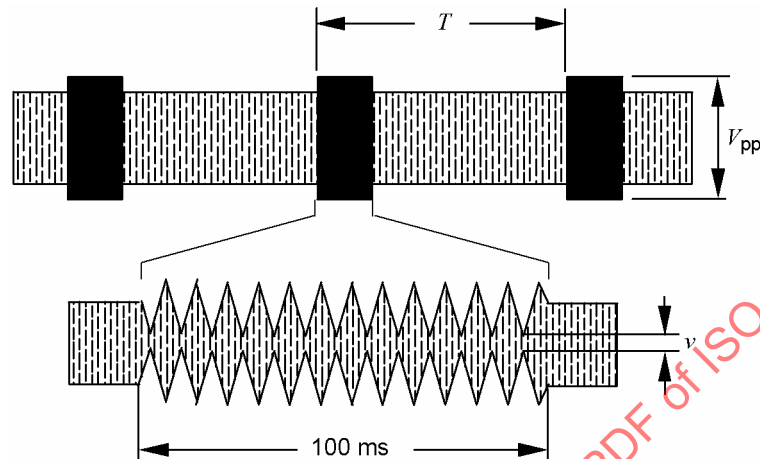
Figure 135 — Test signal for frequencies between 150 kHz and 10 MHz
