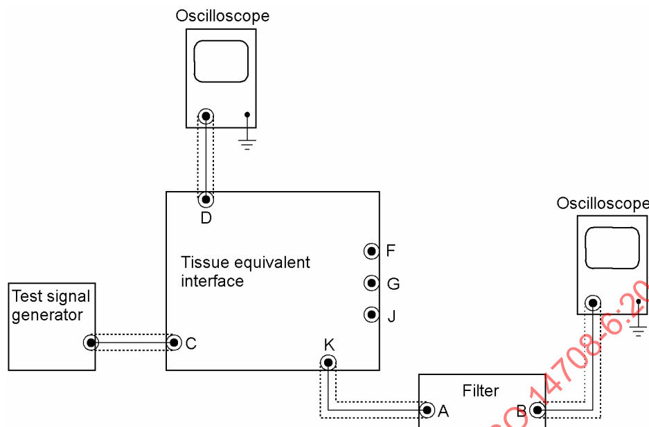
Figure 118 — Test set-up for measurement of induced current flow
