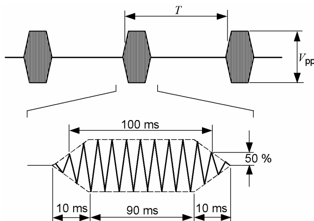
Figure 134 — Modulation 2 (alternative)
