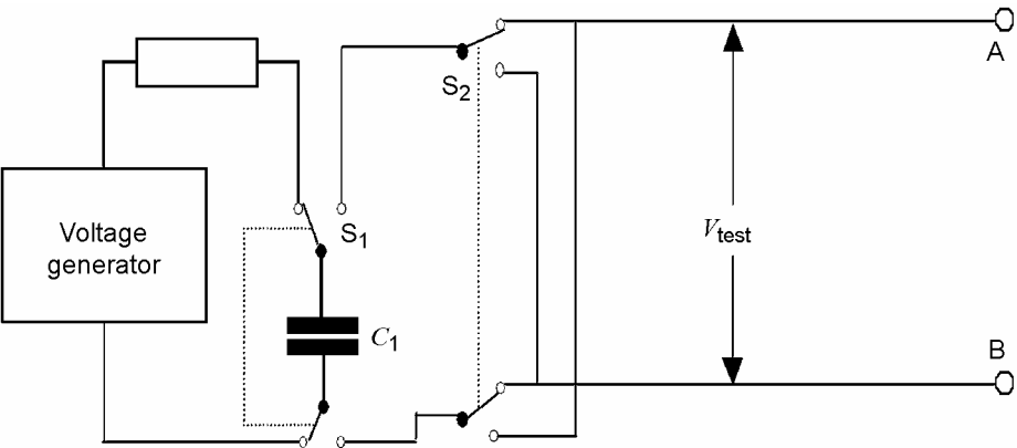
Figure 111 — Test set-up for truncated exponential DEFIBRILLATION waveform
