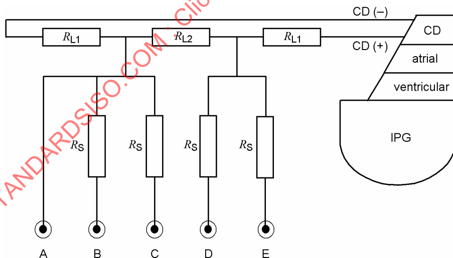
Figure 106 — Test set-up for checking internal DEFIBRILLATION protection
