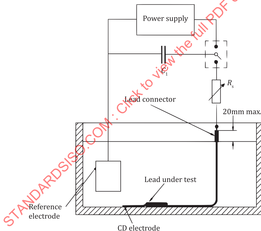
Figure 7 — Conductor current integrity test fixture
