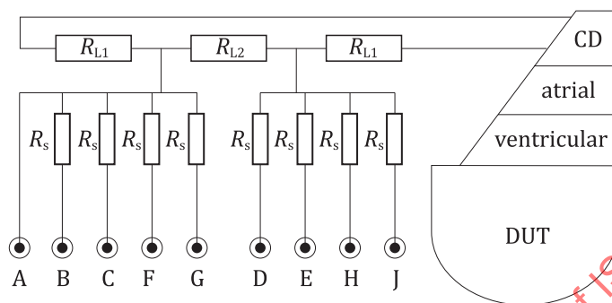
Figure 6 — Example test set-up for checking internal defibrillation protection in a CRT-D device
