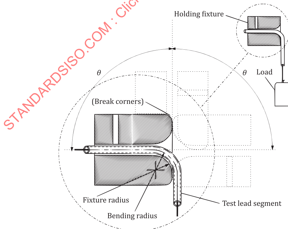
Figure 8 — Conductor flex test fixture
