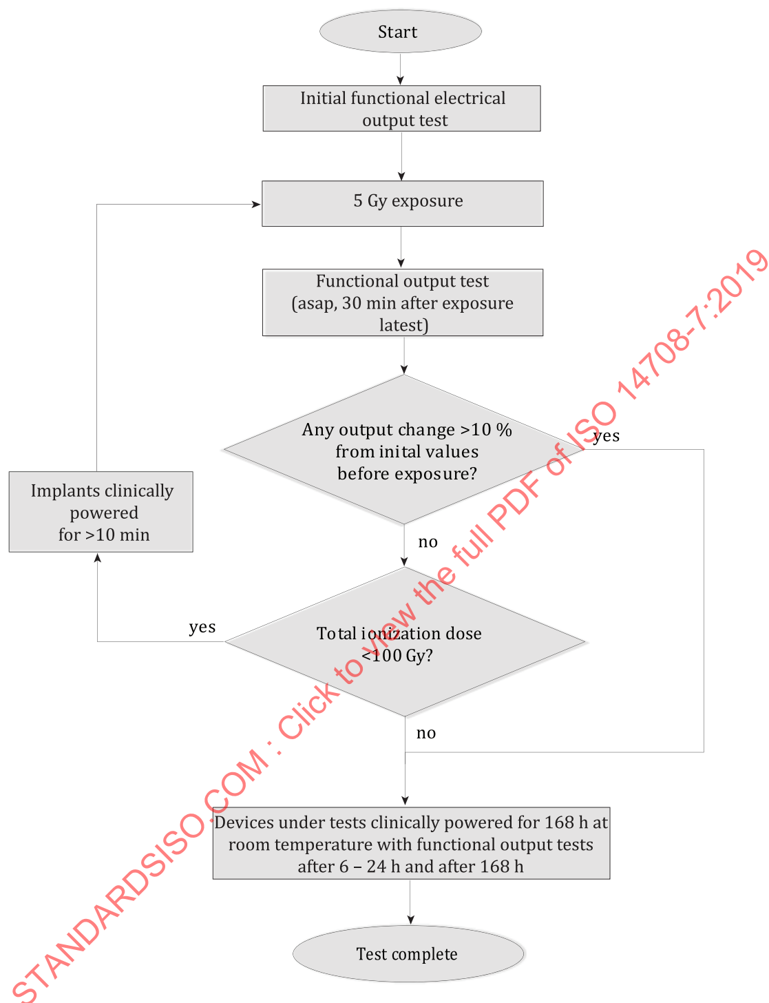
Figure 5 — Flowchart for ionizing radiation robustness test
