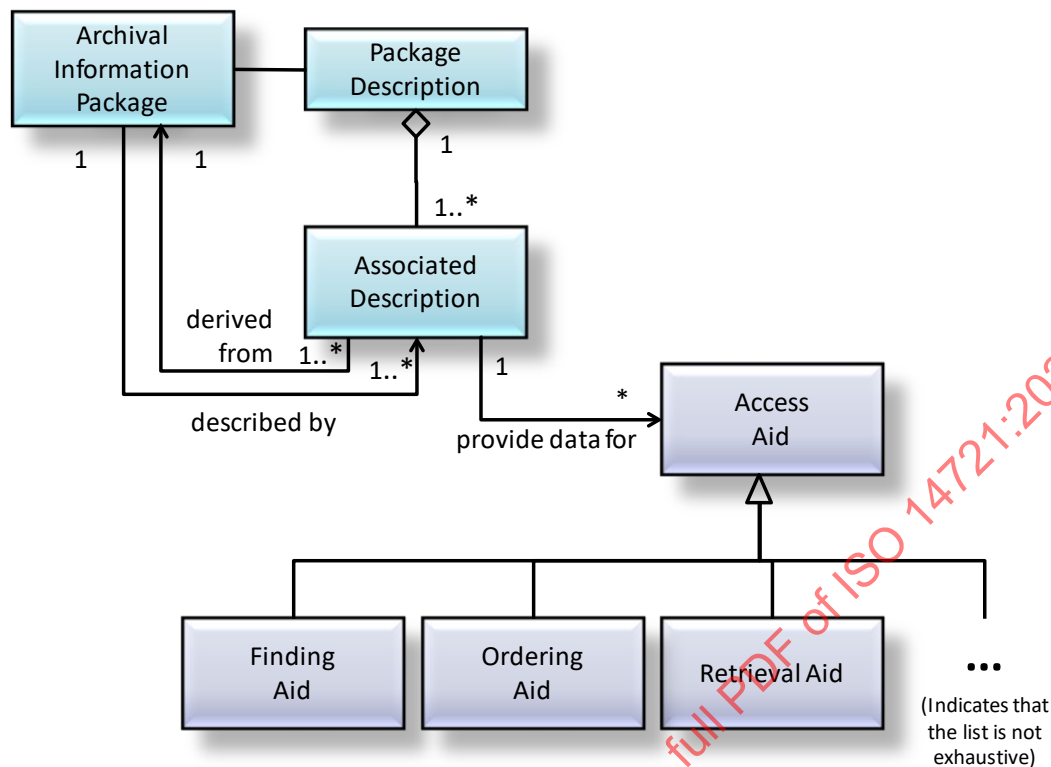
Figure 4-20: Package Description and Its Associated AIP
