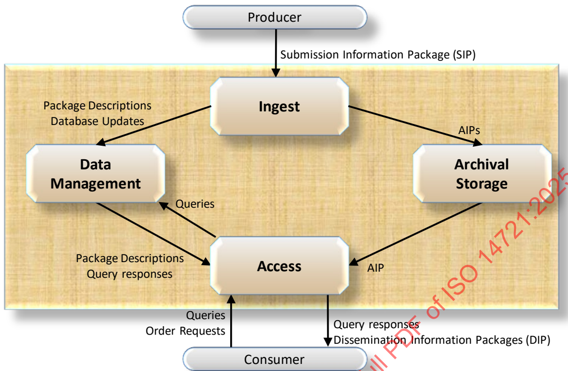
Figure 4-29: High-Level Data Flows in an OAIS
