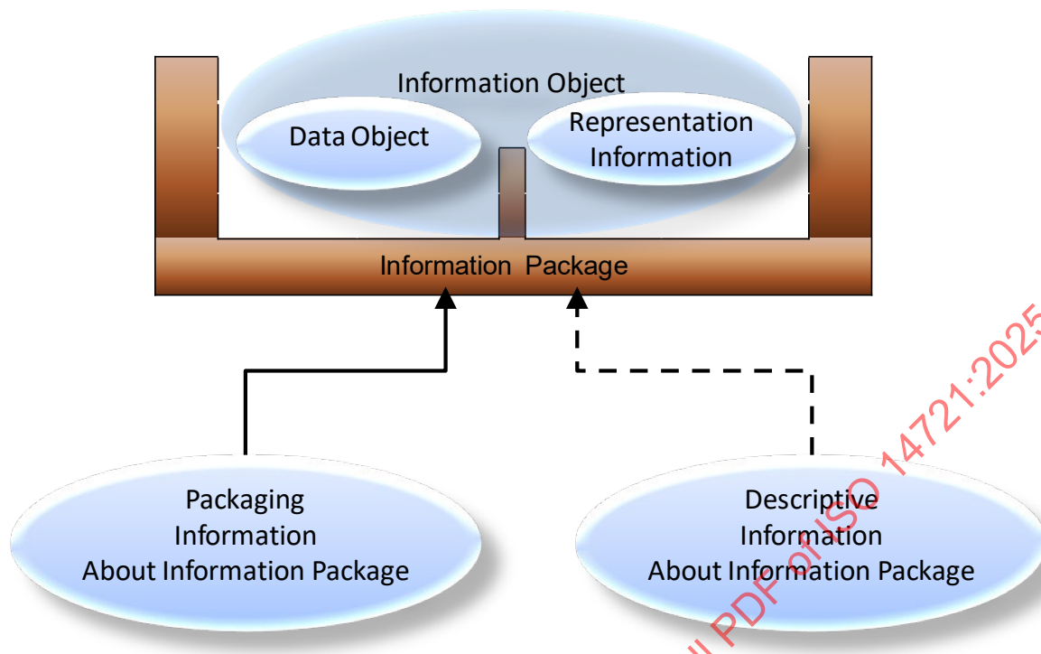
Figure 2-3: Information Package Concepts and Relationships
