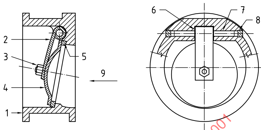
Figure 8 — Single-plate wafer-type check valve, long pattern
