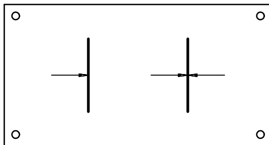
Figure 13 — Typical identification plate for valve with one seat uni-directional and one seat bi-directional
