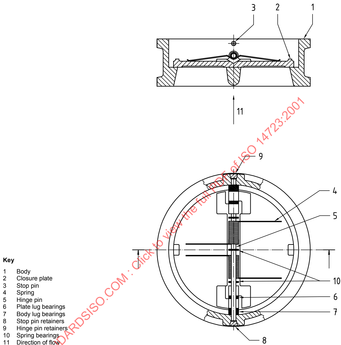
Figure 9 — Typical dual-plate wafer-type check valve, long pattern
