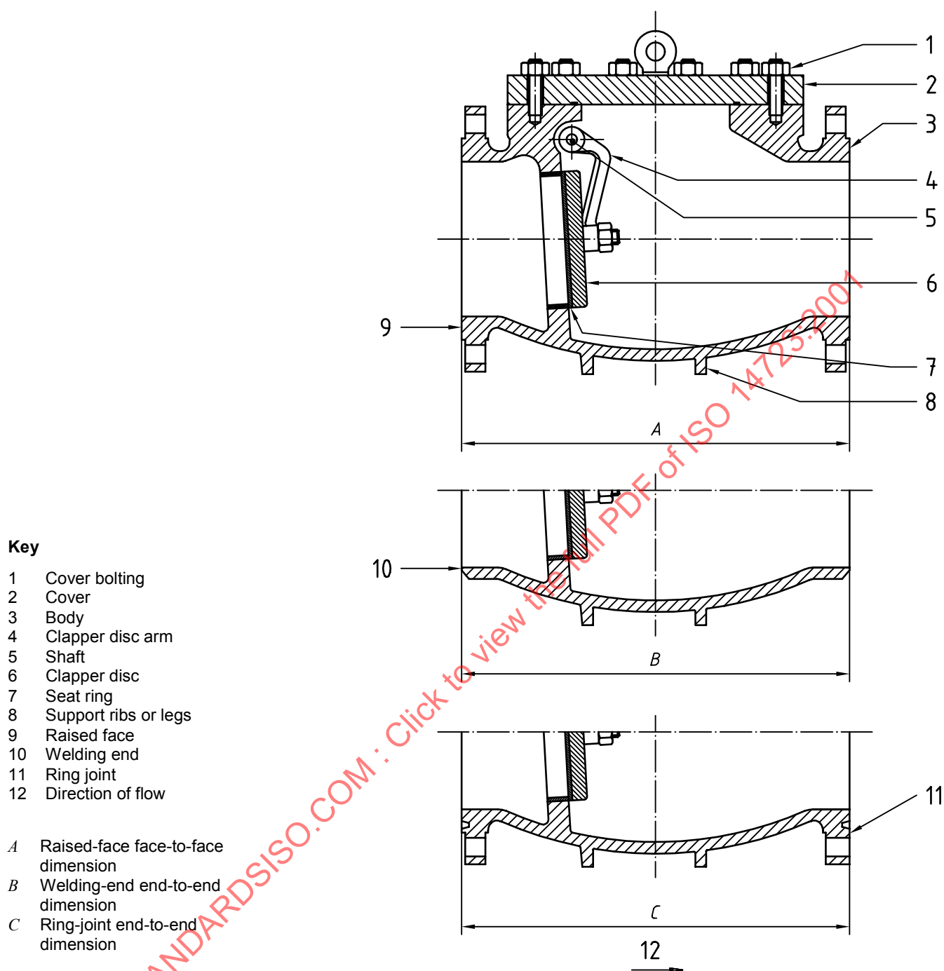
Figure 6 — Reduced-opening swing check valve
