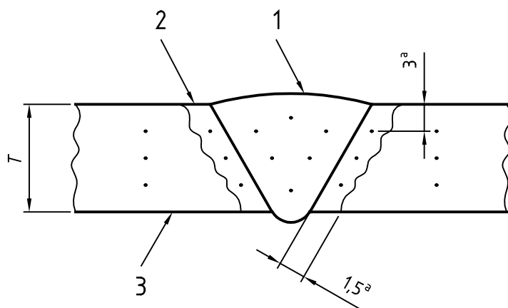
Figure 12 — Hardness survey specimen location
