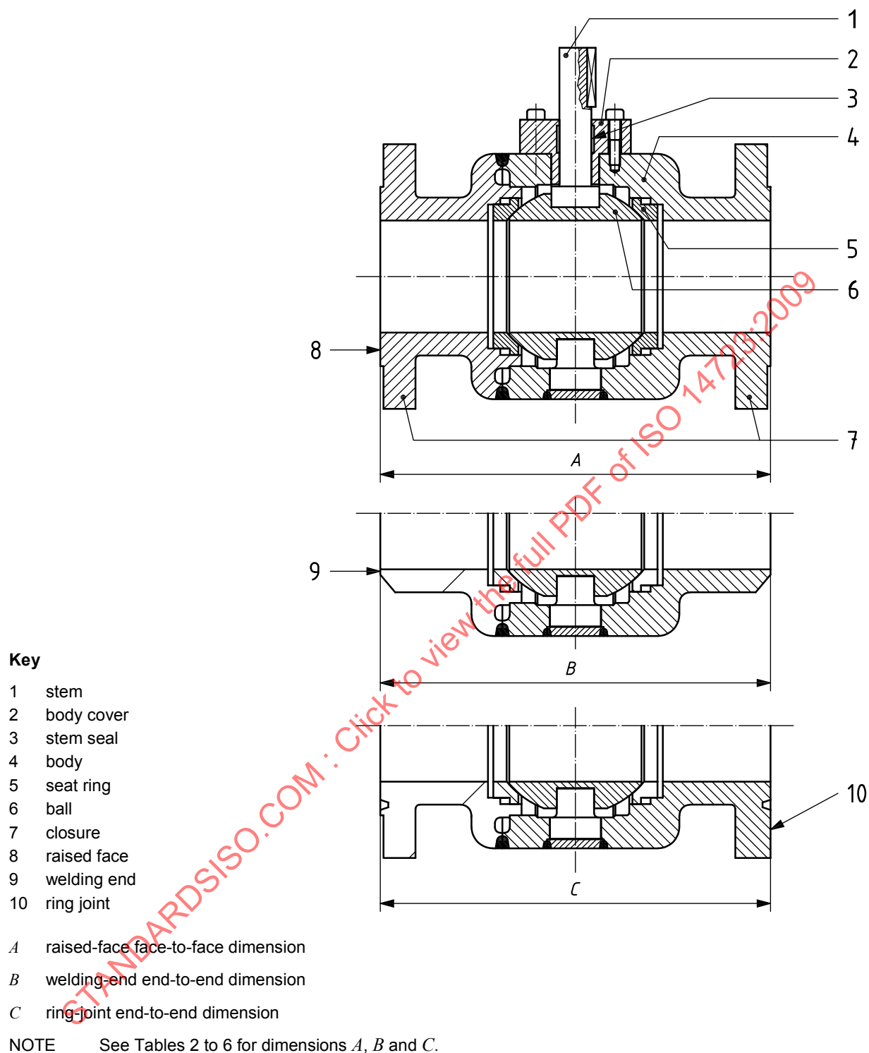
Figure 6 — Typical welded-body ball valve
