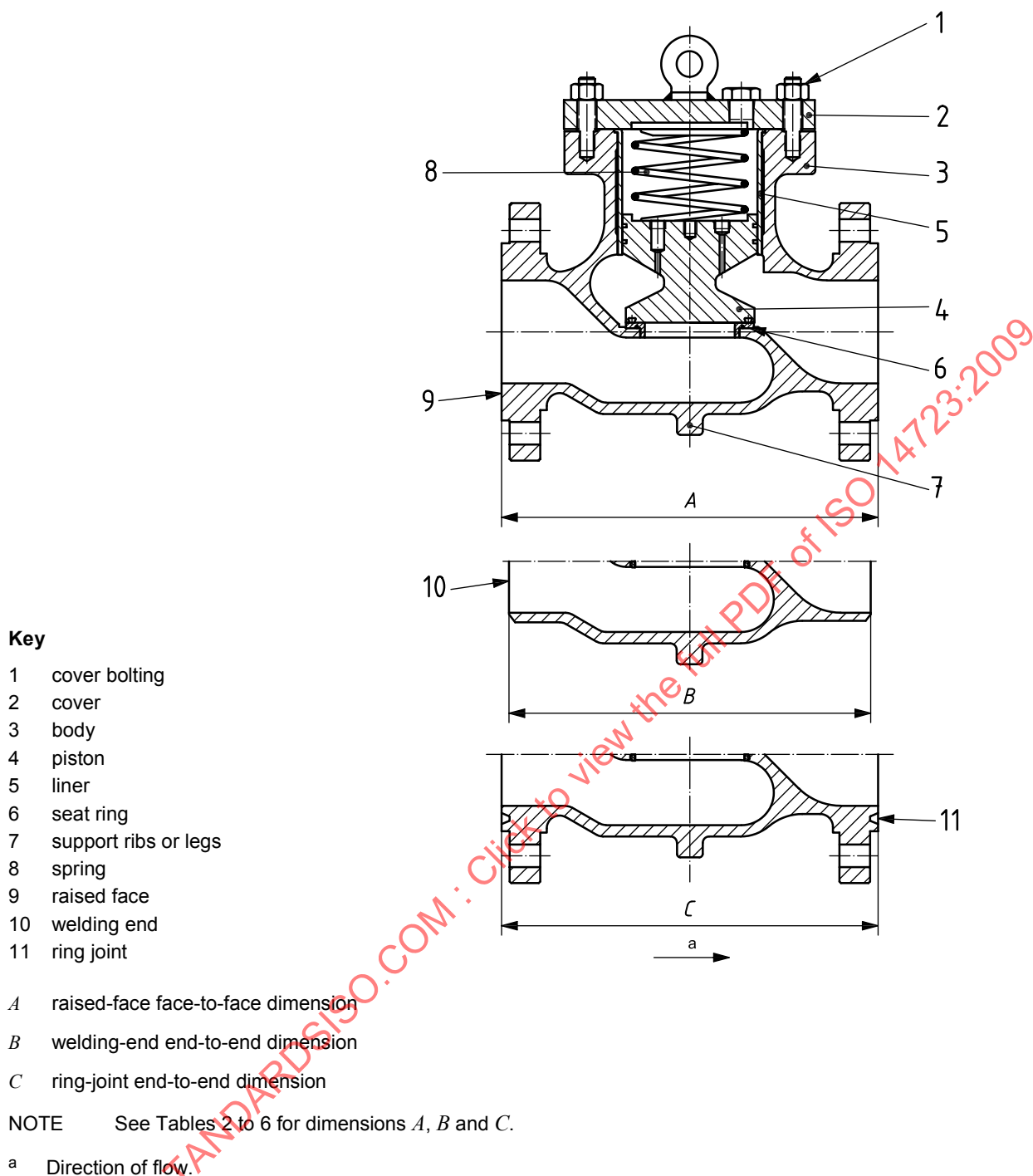
Figure 13 — Typical piston check valve
