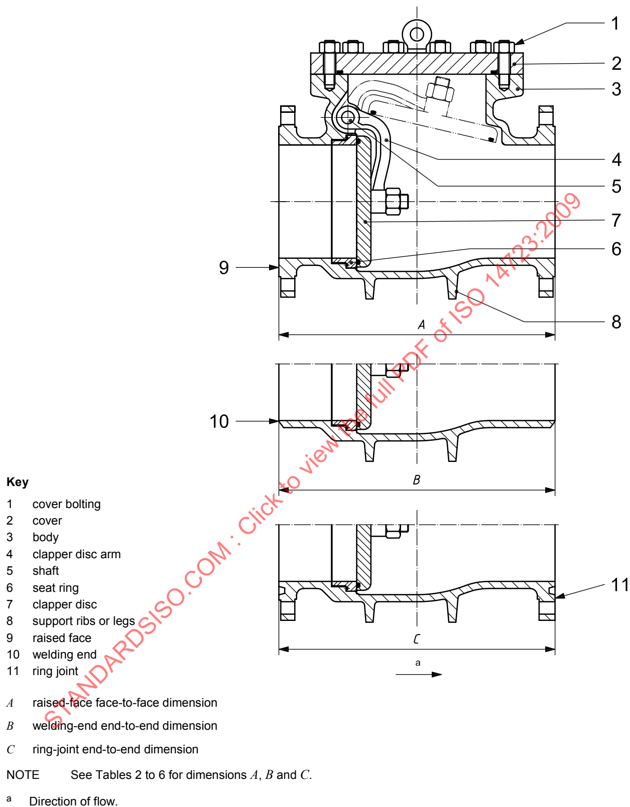
Figure 8 — Typical full-opening swing check valve
