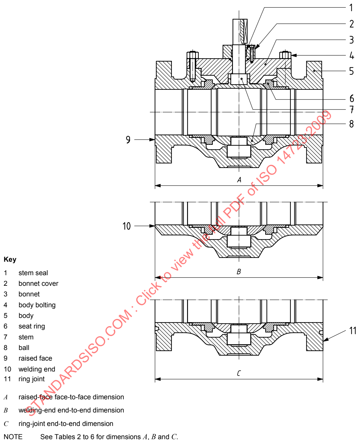
Figure 4 — Typical top-entry ball valve
