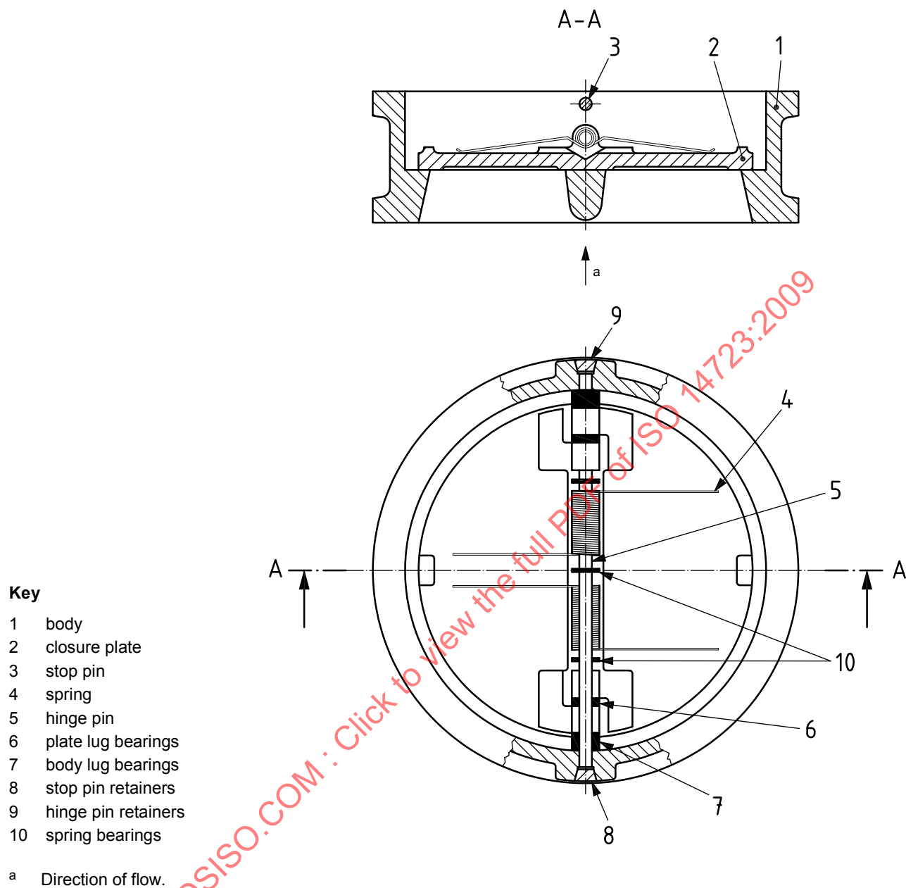
Figure 10 — Typical dual-plate wafer-type check valve, long pattern
