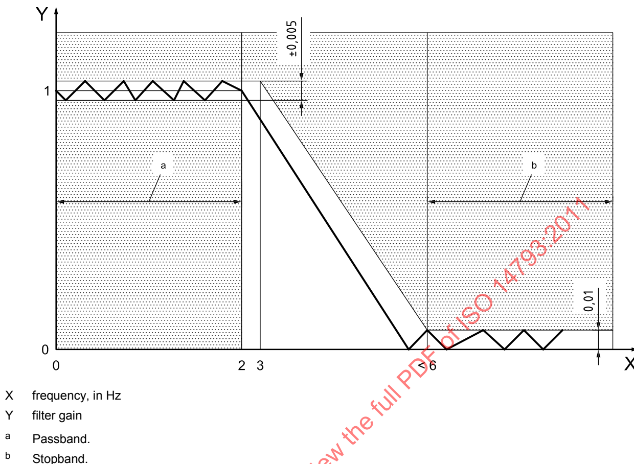
Figure 1 — Required characteristics of phaseless digital filters
