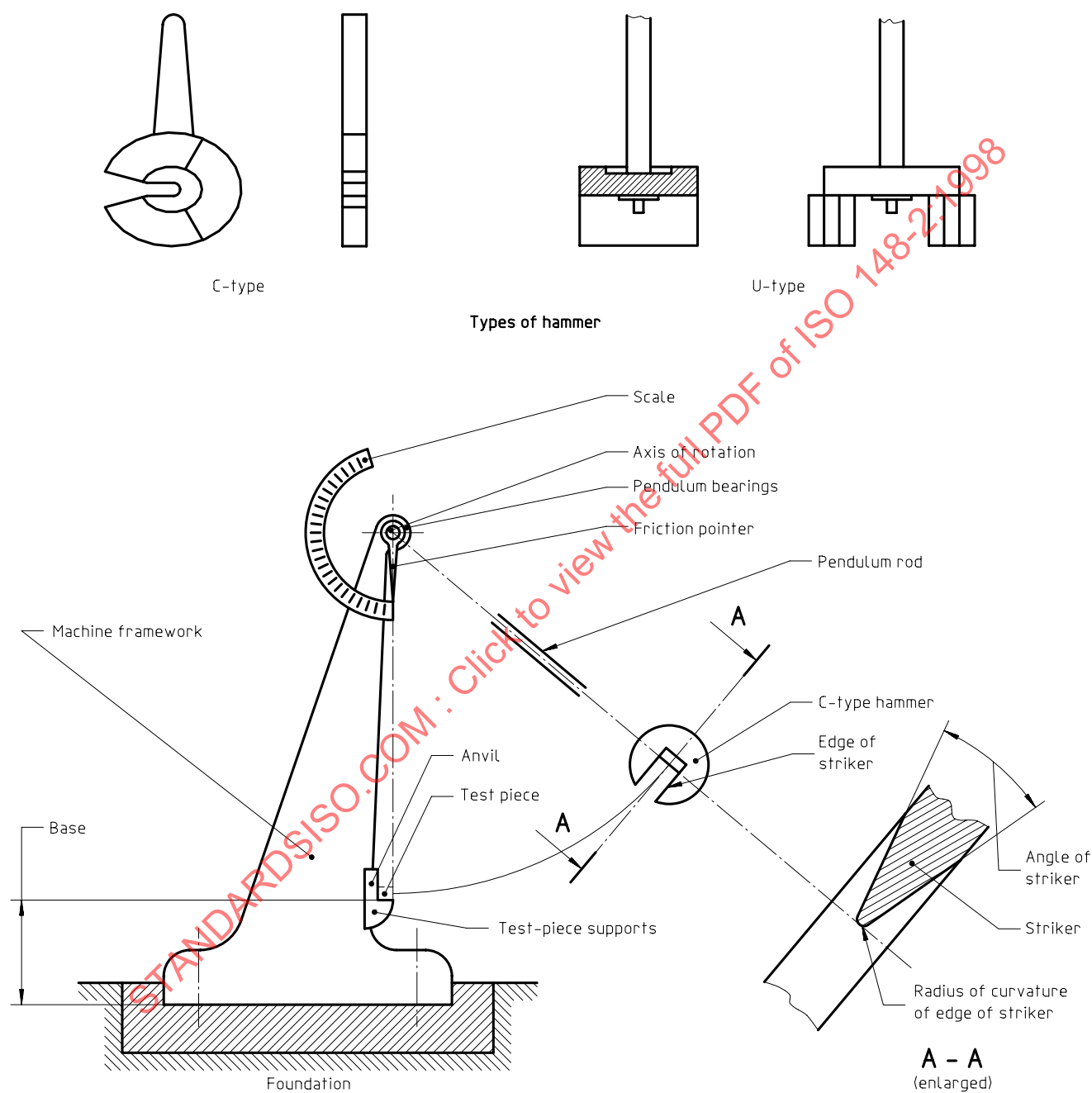
Figure 1 — Parts of a pendulum-type impact test machine
