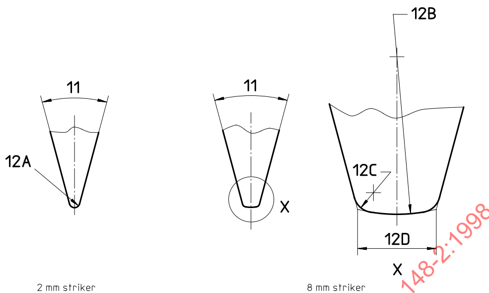
Types of striker
