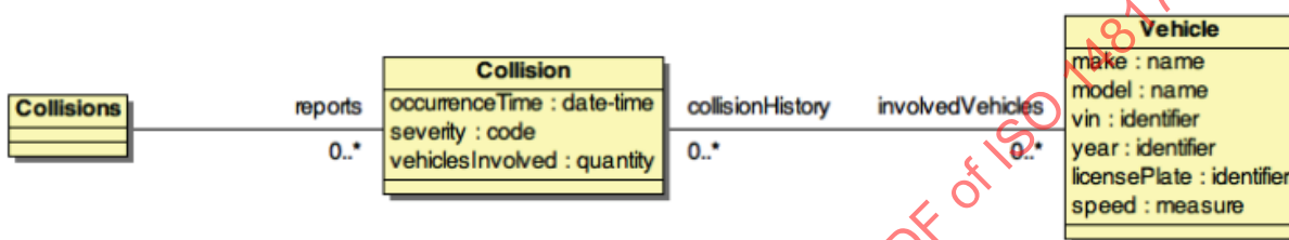
Figure 5 — Sample data model
