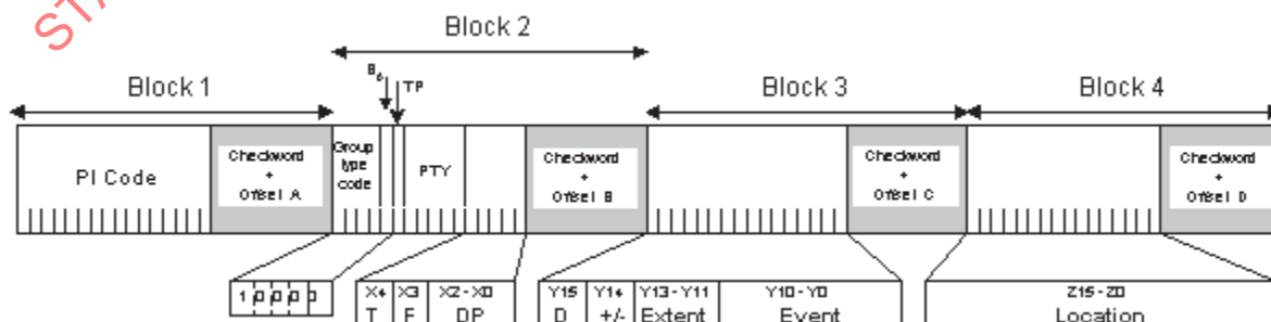
Figure 3 — RDS-TMC single-group full message structure
