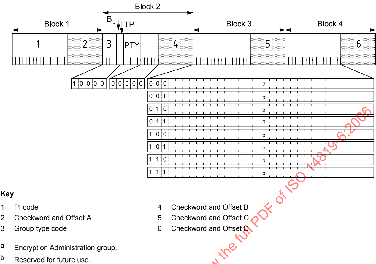
Figure 6 — Type 8A group, used for encrypted RDS-TMC, showing variant usage
