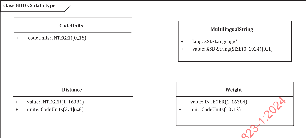
Figure C.4 — Structure of GddDataType
