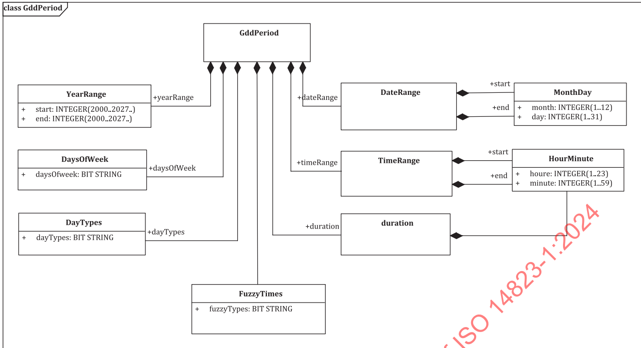
Figure C.2 — Structure of GddPeriod
