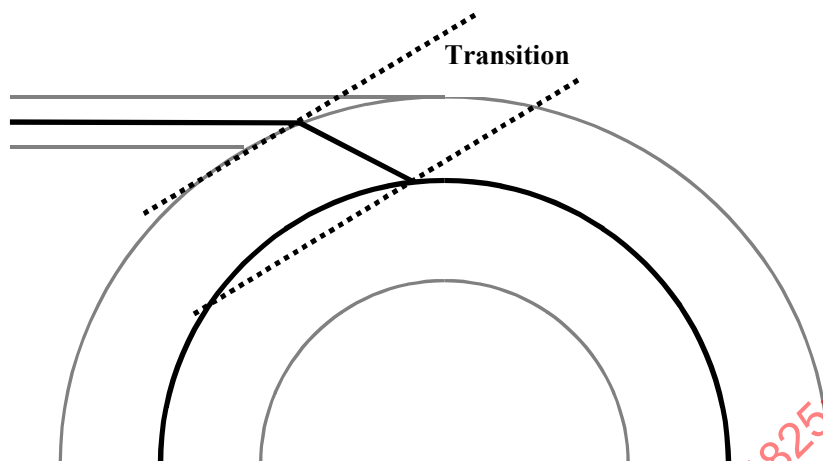
Figure 142 – Schematic example of road centreline transition at a curve/roundabout circle
