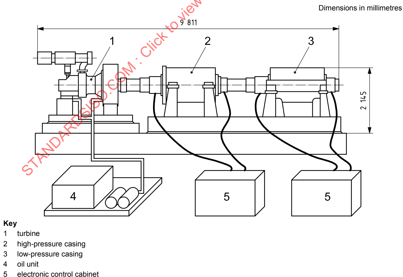
Figure B.1 — Arrangement of a centrifugal compressor set with AMBs
