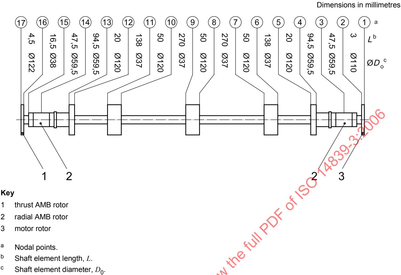
Figure A.2 — Structure of the flexible rotor
