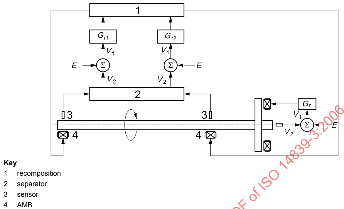
Figure A.7 — Centralized control (MIMO/mode control)
