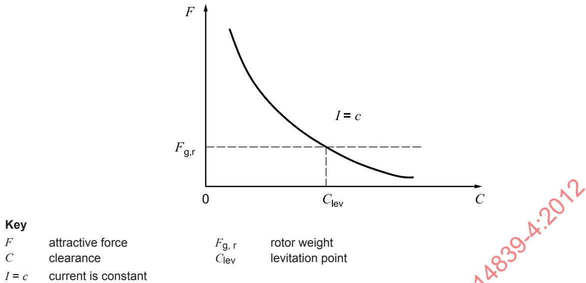
Figure 2 — Relationship between attractive force and clearance when the current is constant
