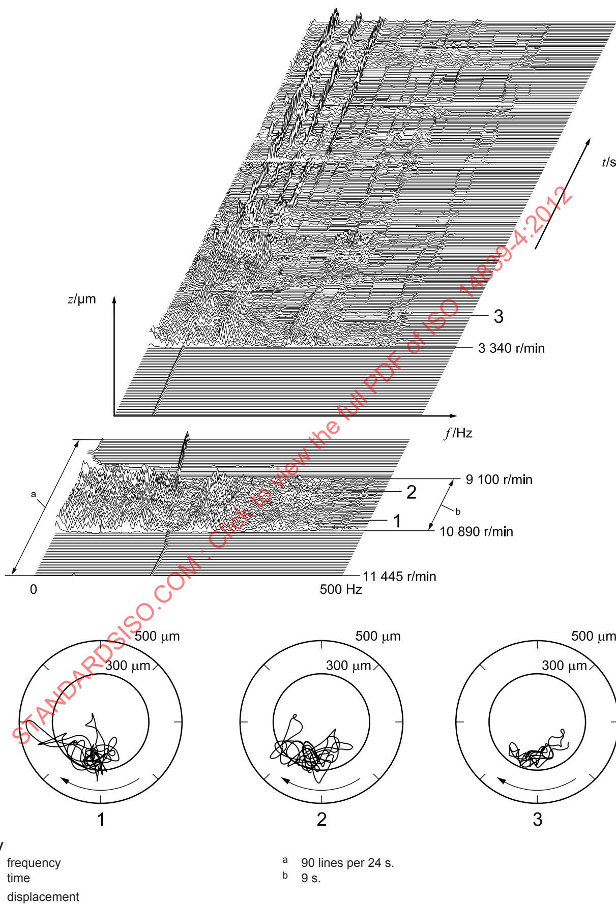
Figure D.1 — Example of touchdown test results
