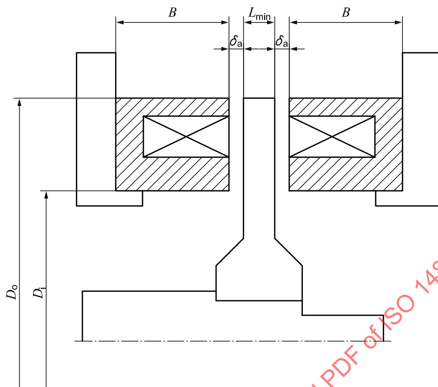
Figure A.2 — Shape of a thrust magnetic bearing
