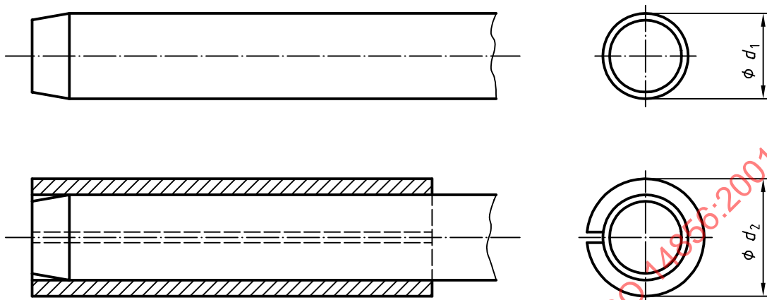
Figure 3 — Fastening pin and slit tube
