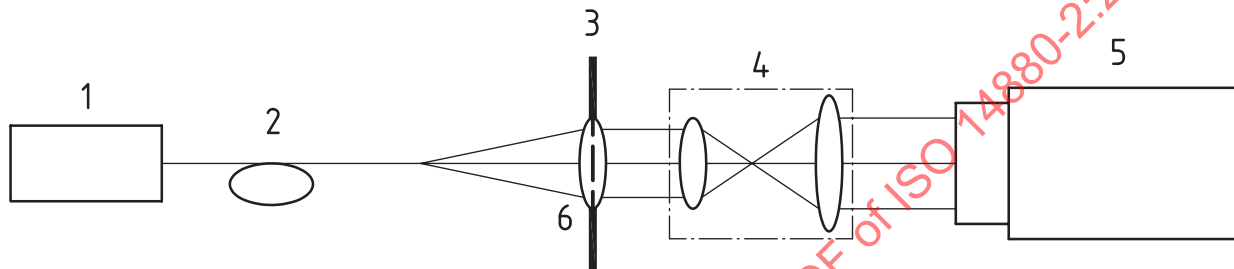
Figure D.1 — Layout for reference measurement
