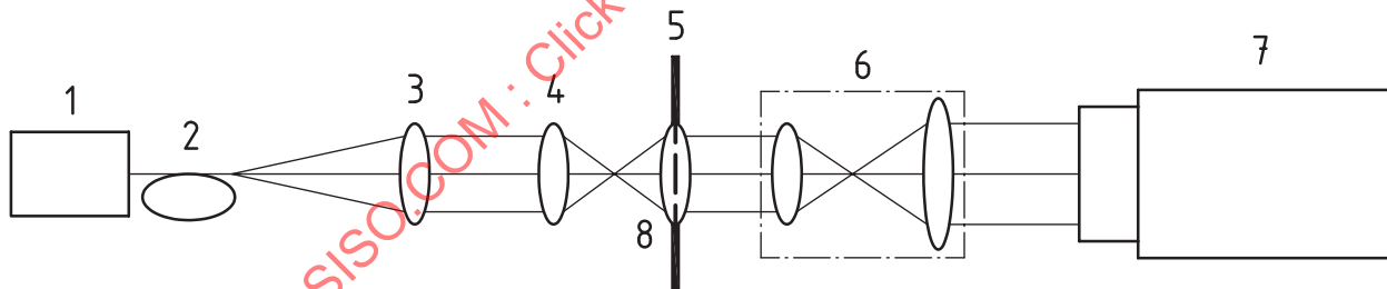
Figure D.2 — Layout for measurement of a "slow" microlens
