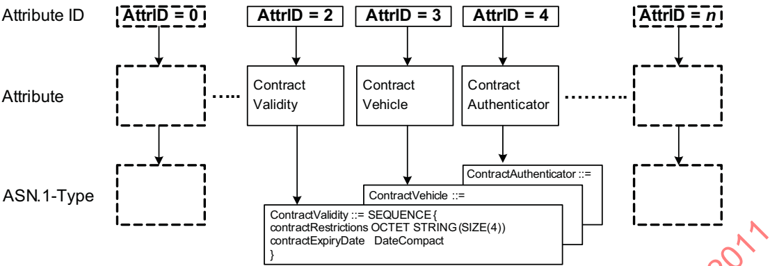
Figure 3 — Basic addressing mechanism
