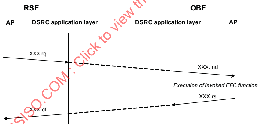
Figure 8 — The logical sequencing of service primitive exchanges
