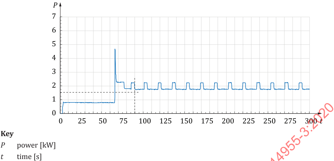
Figure A.2 — Measurement of power during machine tool state OFF to STANDBY
